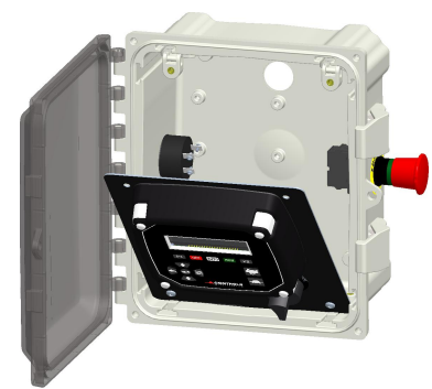
HINGED CORNER MOUNTS ALLOW EASY 2-SCREW CONNECTOR ACCESS SCALE 0.125
